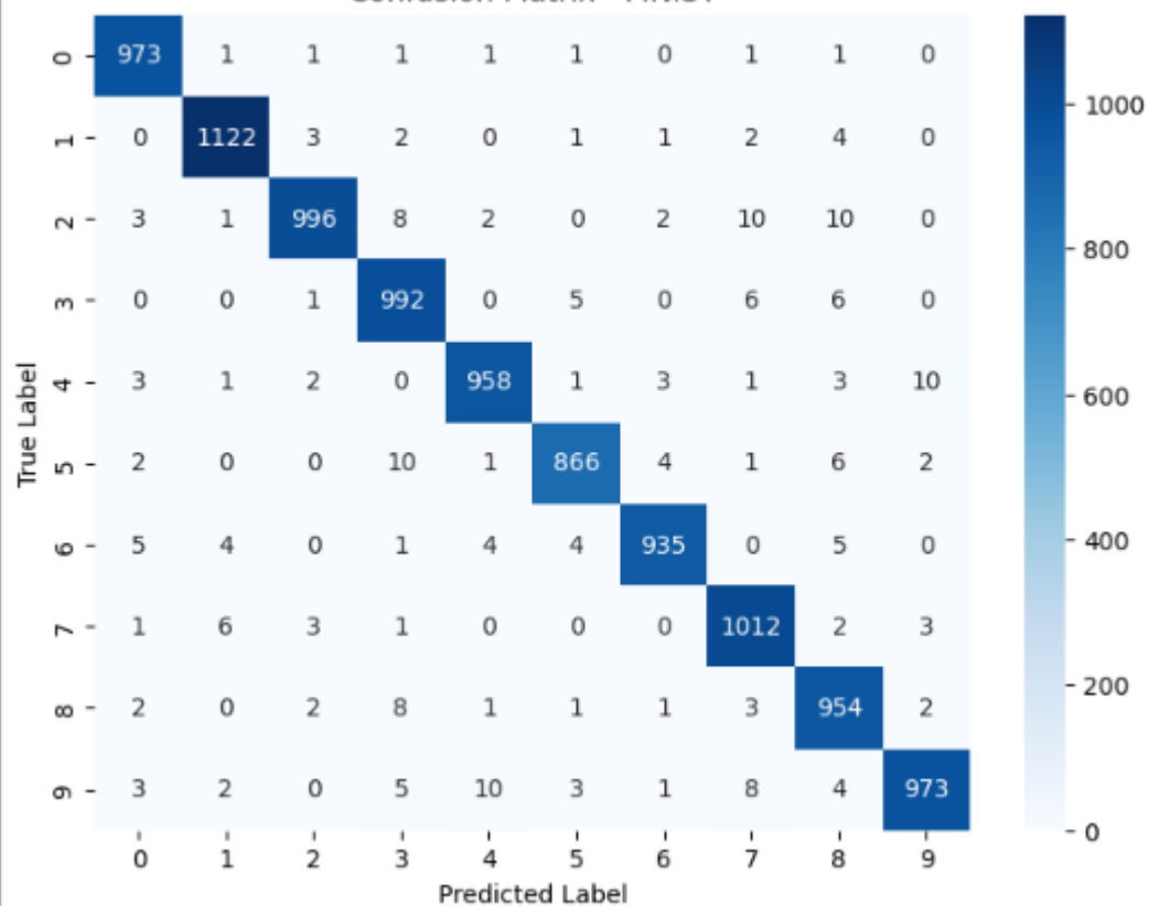
Confusion Matrix - MNIST
